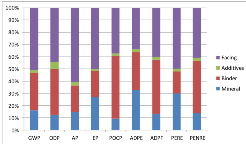
Figure 3: Shares of the different raw materials in the whole raw material supply (A1) of İzocam Stonewool production
