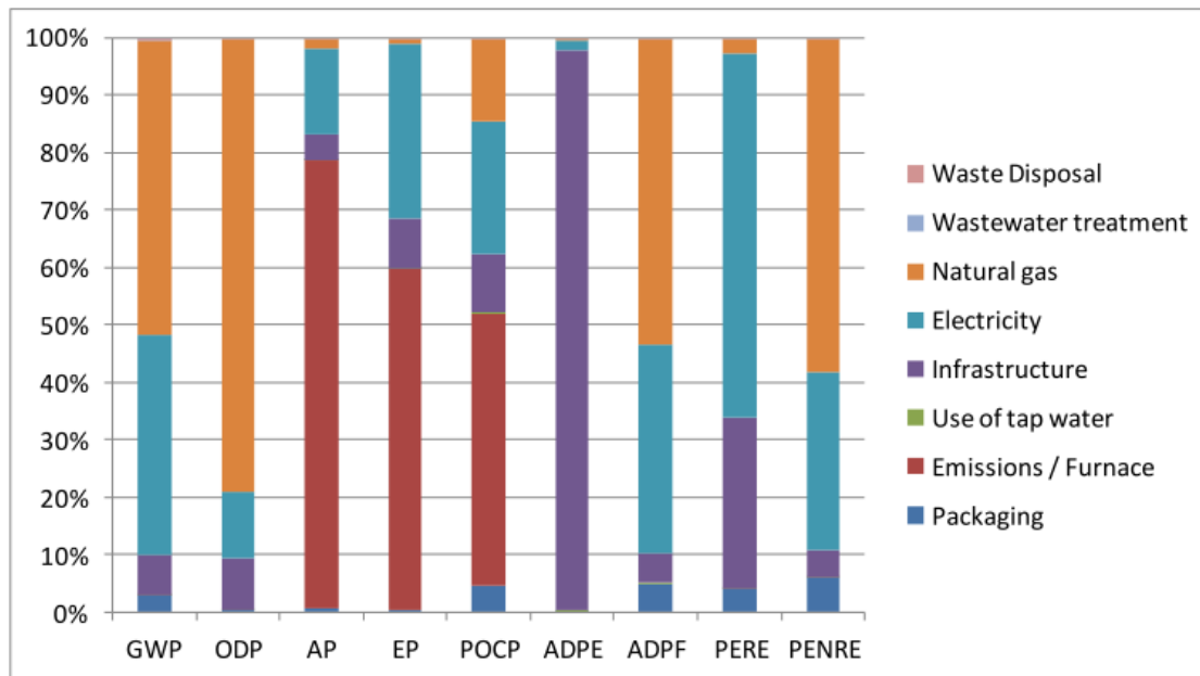
Figure 4: Load components in manufacturing (A3) of İzocam Stonewool insulation materials
