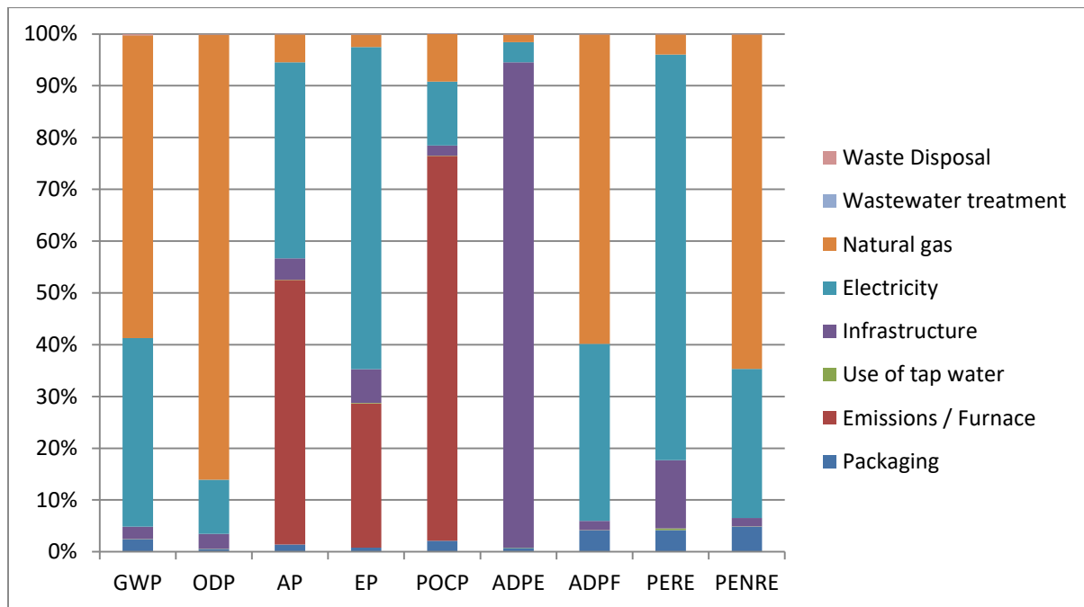
Figure 4: Load components in manufacturing (A3) of İzcam Glasswool insulation materials
