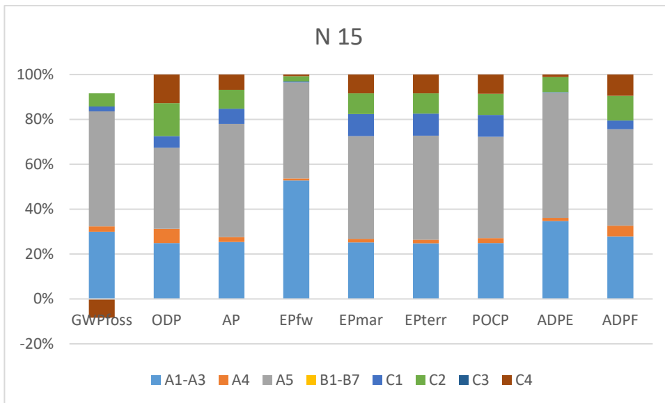
Figure 3: Share of life cycle stages in the overall result using the example of the product N 15
