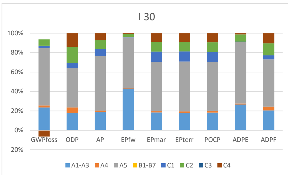
Figure 4: Share of life cycle stages in the overall result using the example of the product I 30
